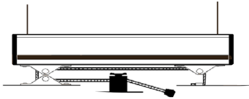
DOUBLE PULLEY BOTTOM RAIL CONSTANT TENSION SPRING OUTSIDE RECESS ONLY
